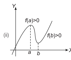
Figure 8.38 f(x) has one real root
