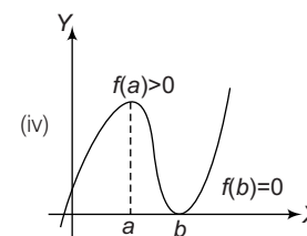
Figure 8.40 f(x) has three real roots (b being repeated)
