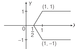
Graph, |y| = f(x) Figure 4.18
