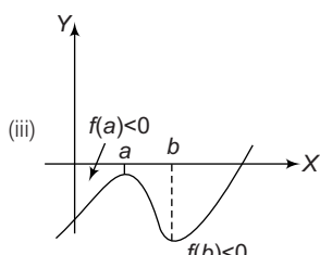
Figure 8.39 f(x) has one real root
