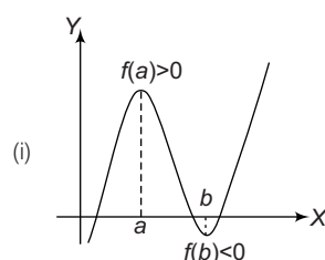
Figure 8.37 f(x) has three distinct roots
