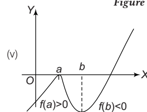
Figure 8.41 f(x) has three real roots (a being repeated)
